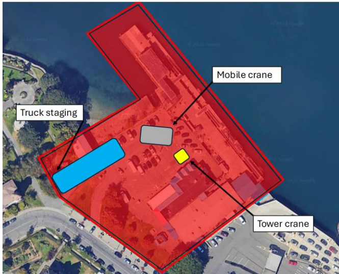
Locations of upcoming tower crane work activities
