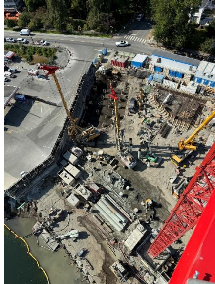
Figure 2: Progressing with final piles for the terminal building.
